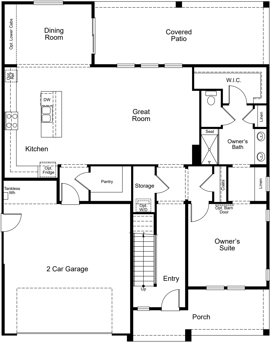
FIRST FLOOR
