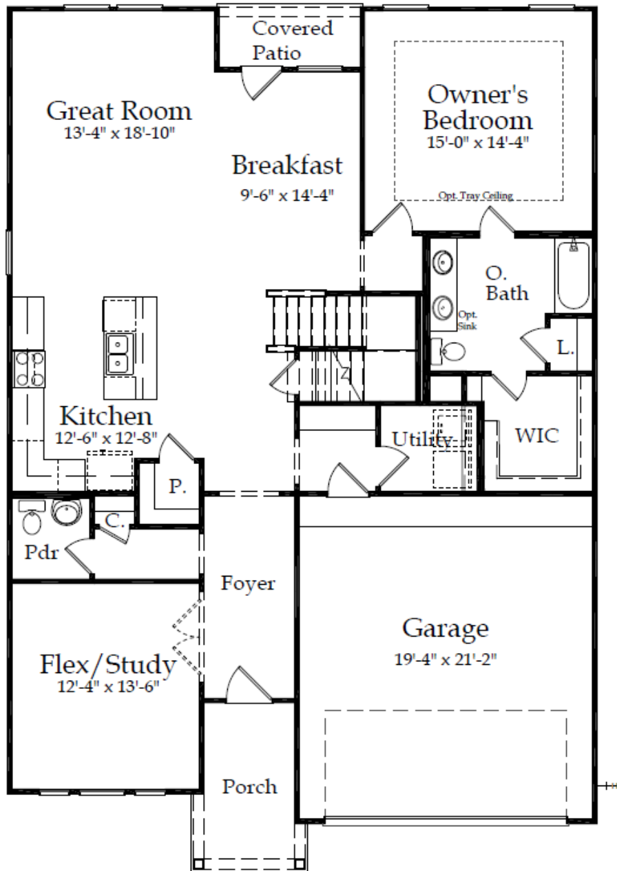
First Floor
