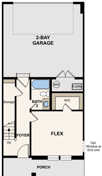
FIRST LEVEL
