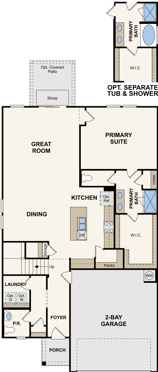
FIRST FLOOR
