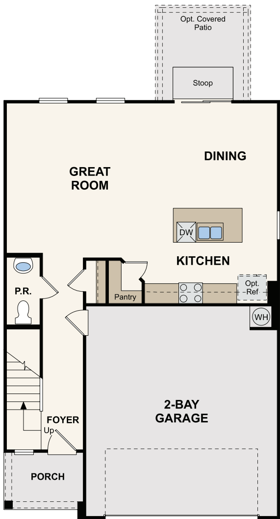
FIRST FLOOR
