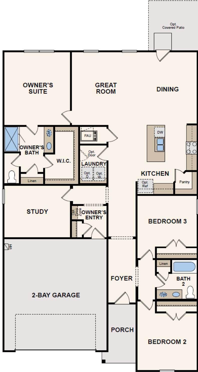
FLOOR PLAN
