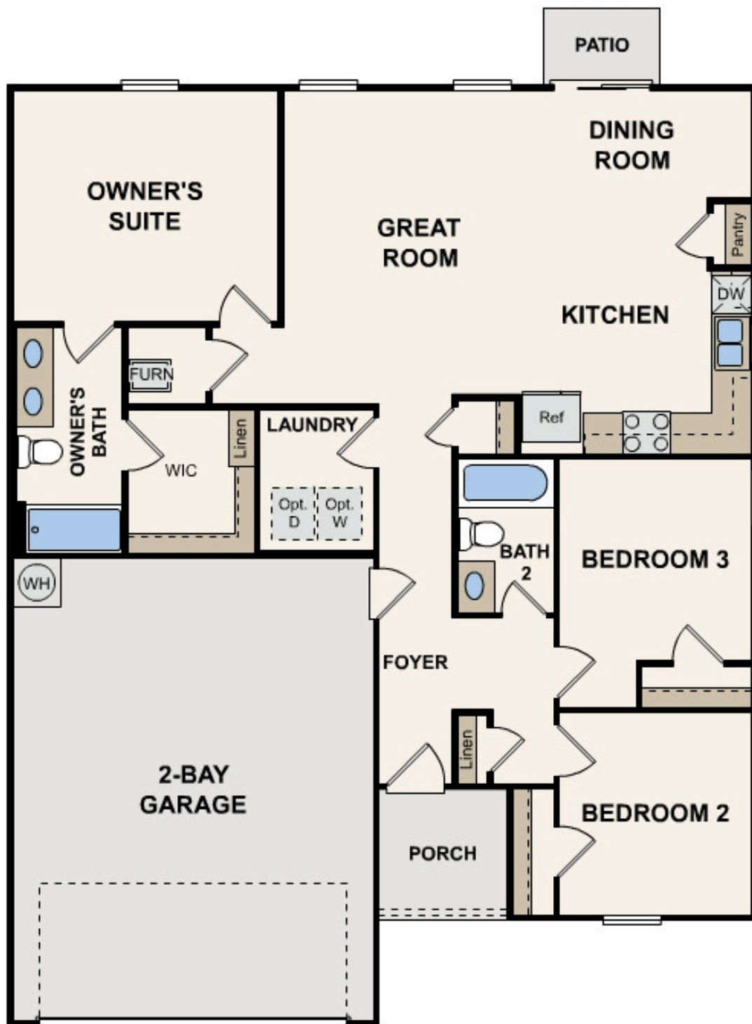
FLOOR PLAN
