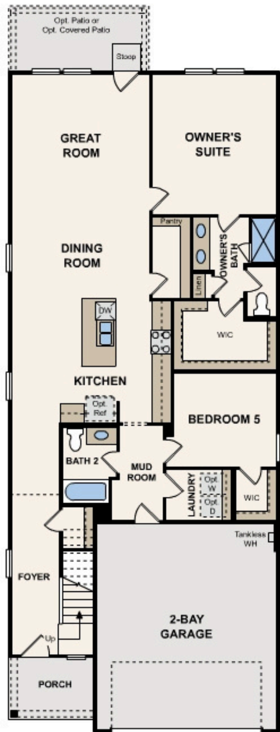
FIRST FLOOR
