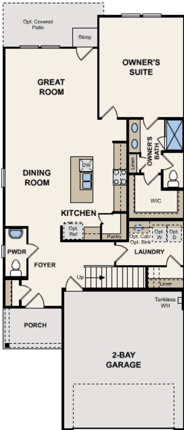
FIRST FLOOR
