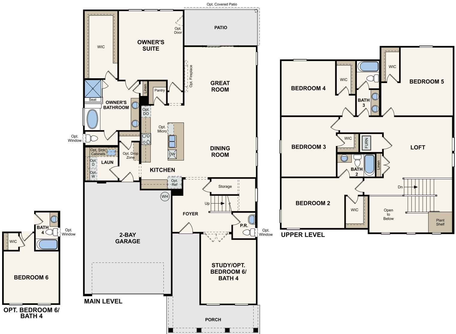
FLOOR PLAN
