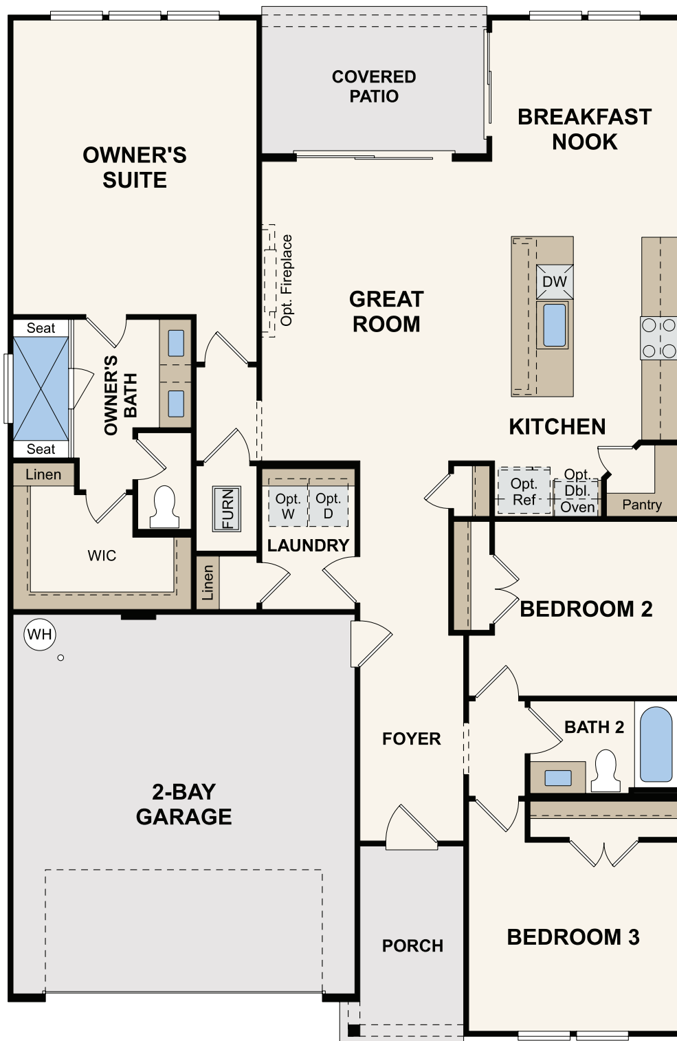
FLOOR PLAN
