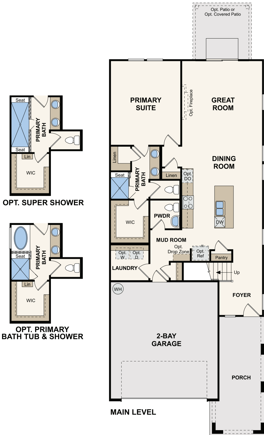
FLOOR PLAN
