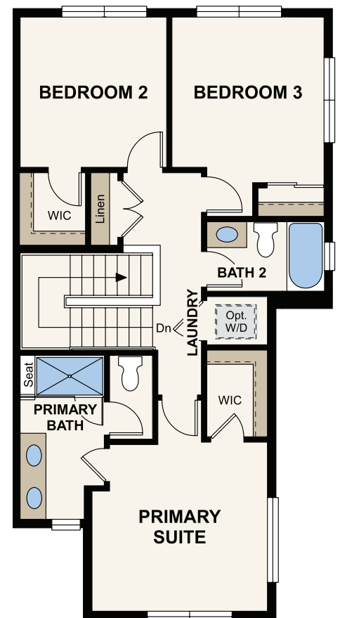
UPPER LEVEL
