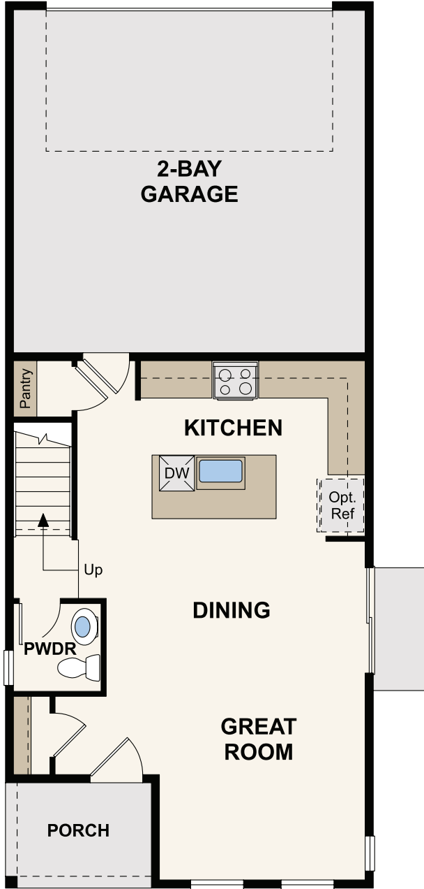
MAIN LEVEL
