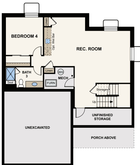
OPT. FINISHED LOWER LEVEL
