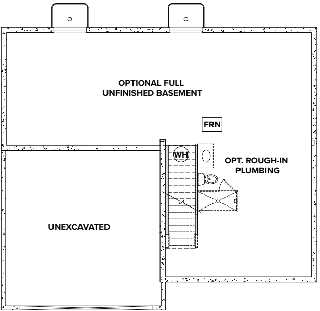
OPTIONAL UNFINISHED BASEMENT
