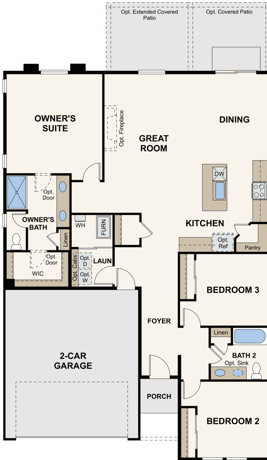
FLOOR PLAN
