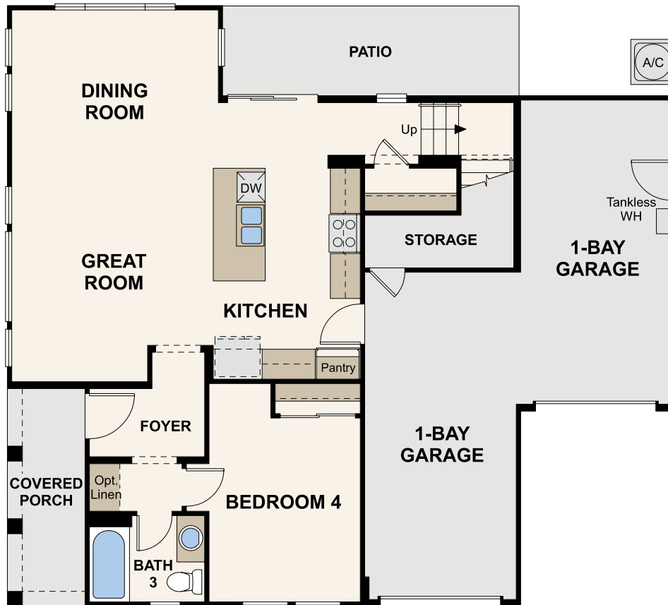
MAIN LEVEL
