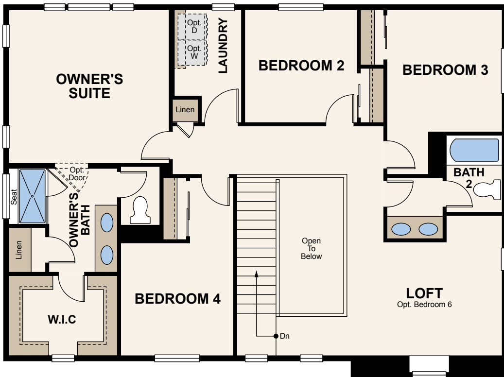
SECOND FLOOR
