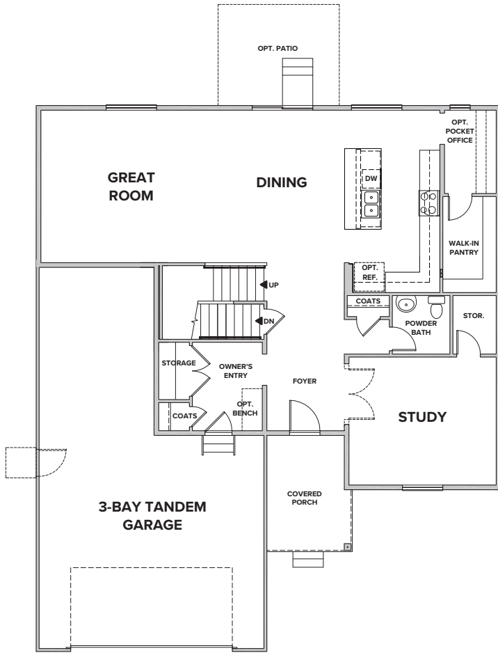
MAIN FLOOR
