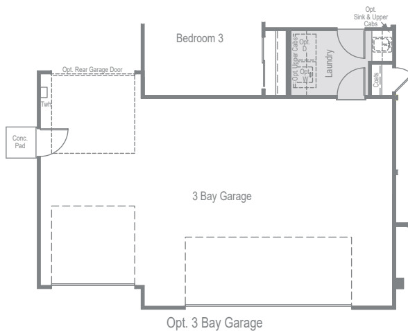
Floor Plan
