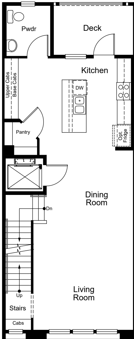
SECOND FLOOR
