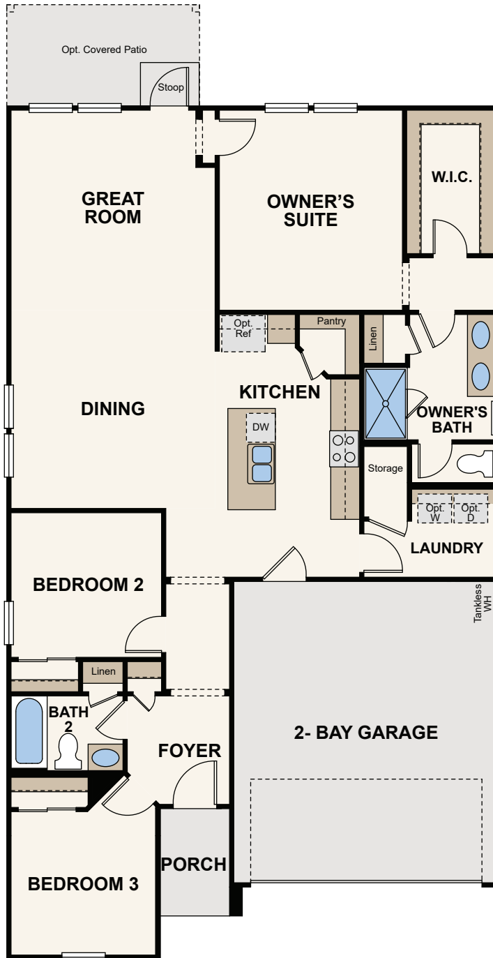
FLOOR PLAN
