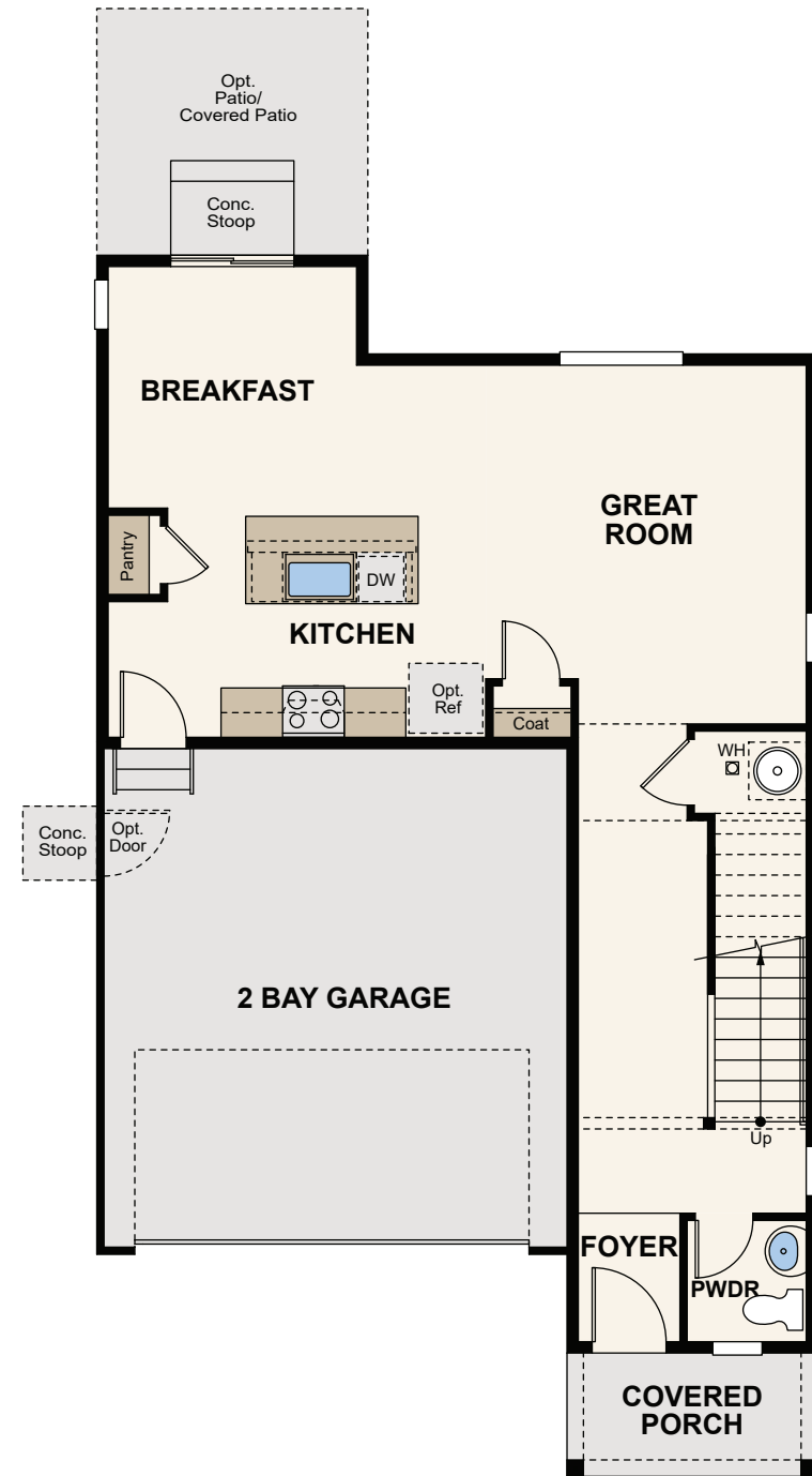
FIRST FLOOR
