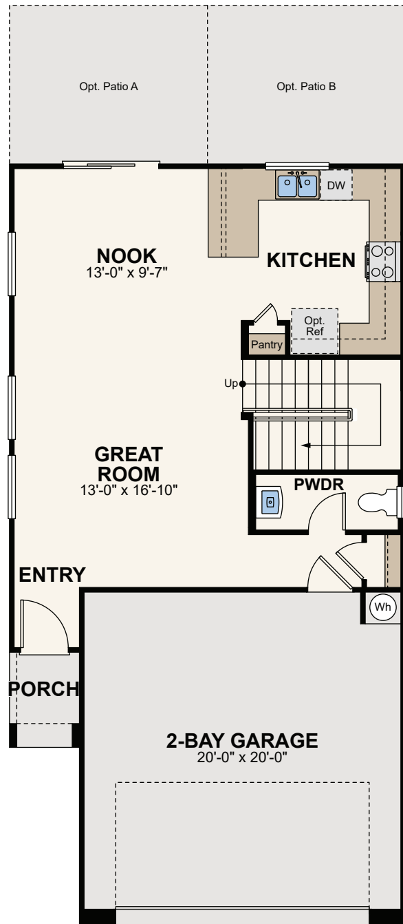
FIRST FLOOR PRELIMINARY
