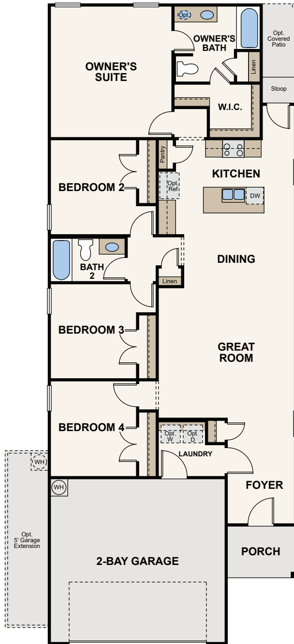
FLOOR PLAN
