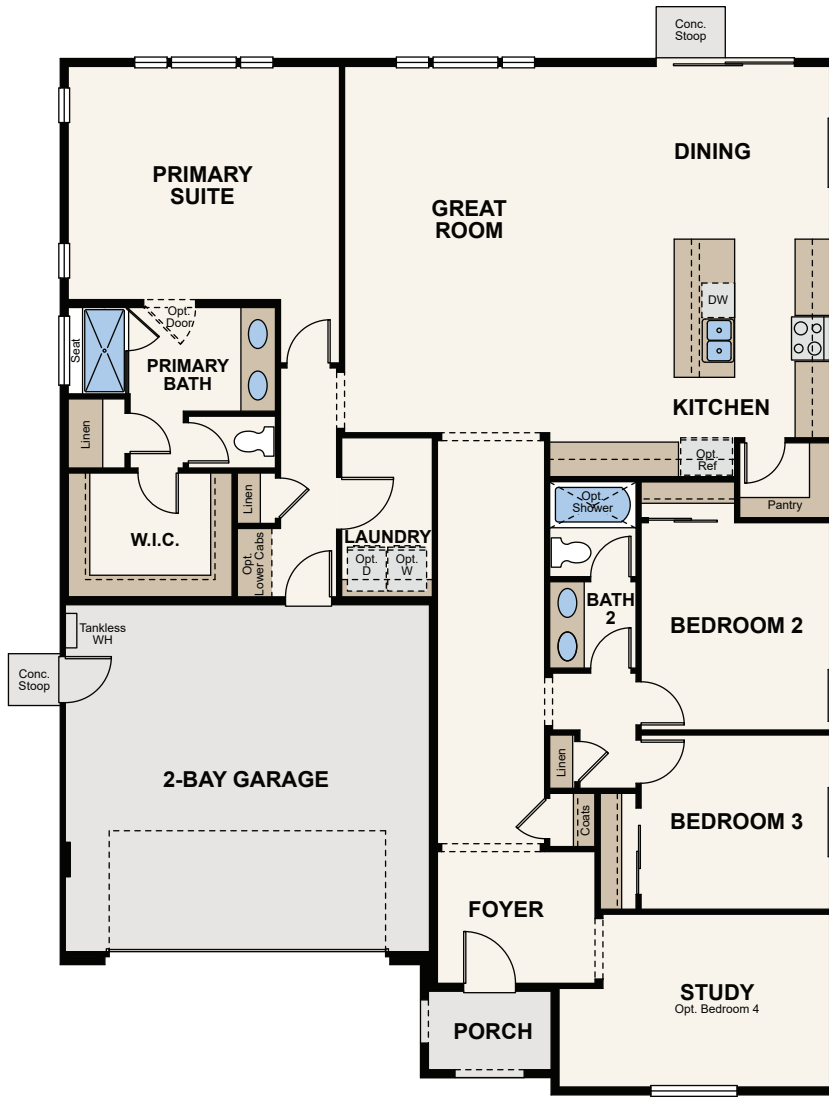
FLOOR PLAN
