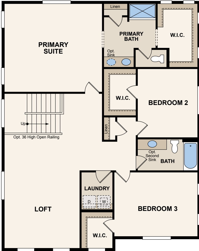
SECOND FLOOR
