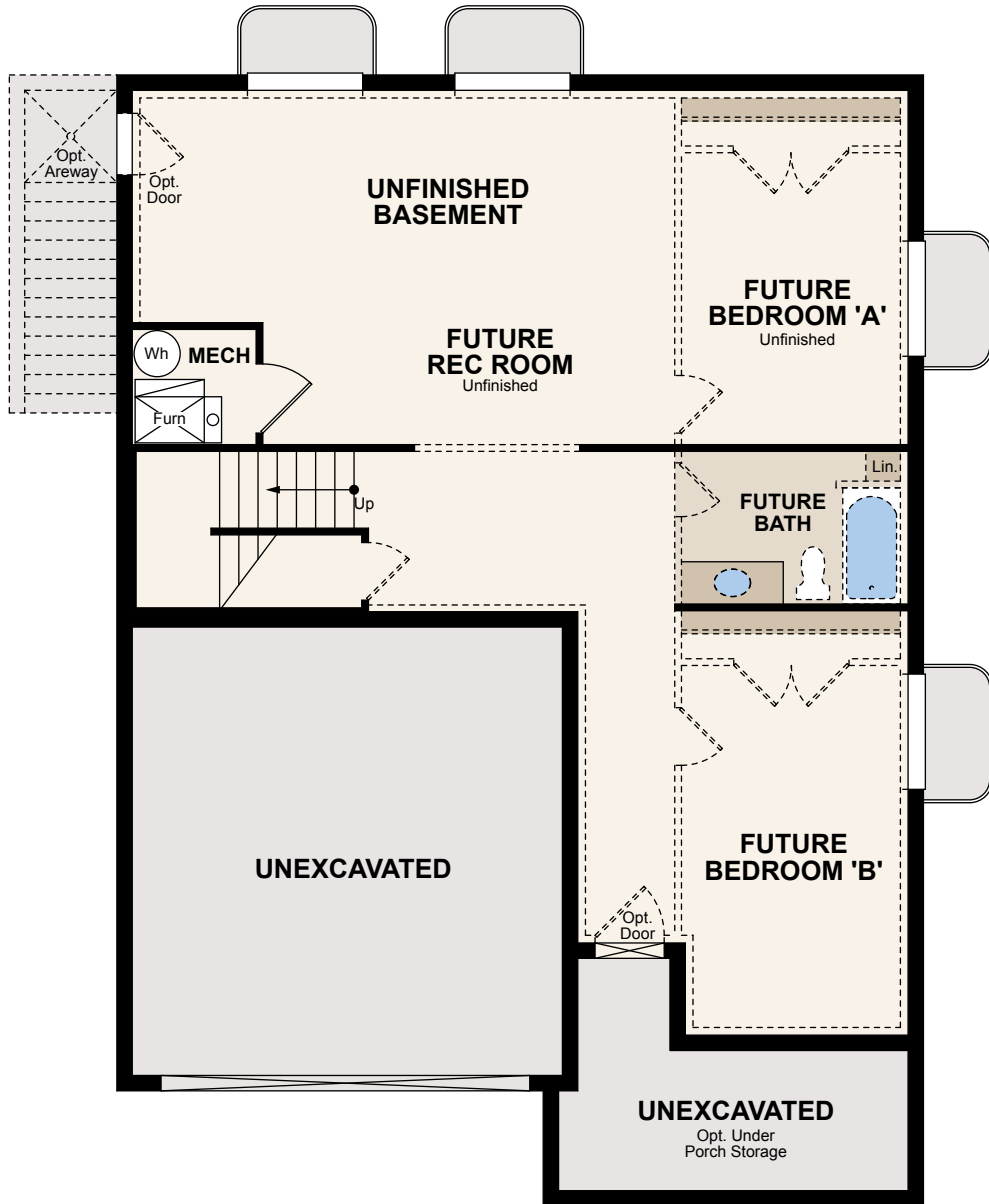
UNFINISHED BASEMENT
