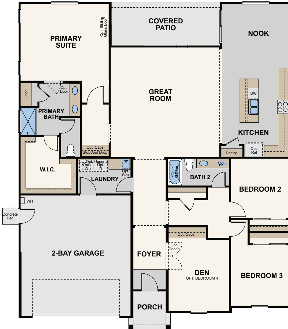
FLOOR PLAN
