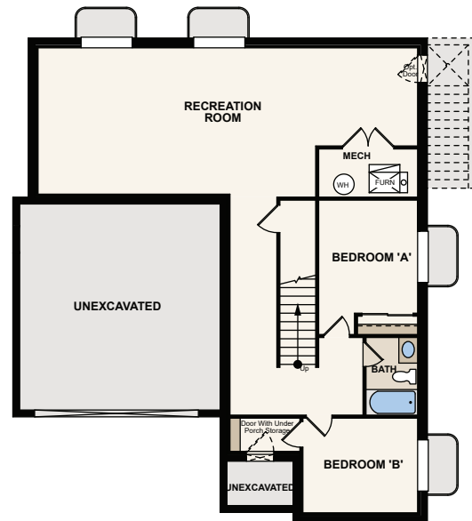
FINISHED BASEMENT
