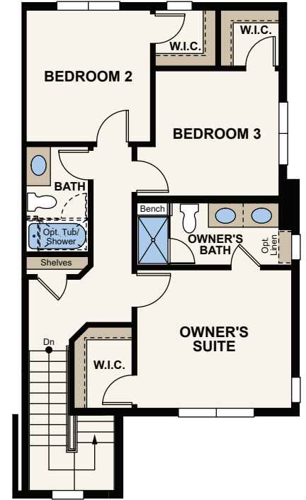
THIRD FLOOR
