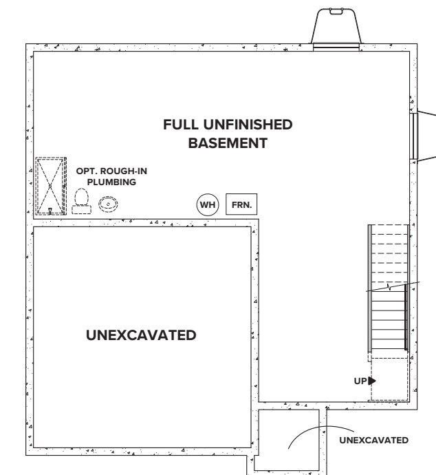
OPTIONAL FULL UNFINISHED BASEMENT
