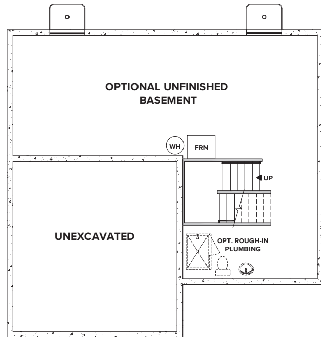
OPTIONAL UNFINISHED BASEMENT
