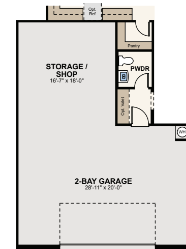
OPT. 5' GARAGE EXTENSION
