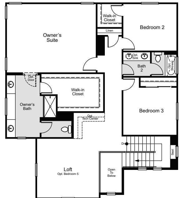
SECOND FLOOR
