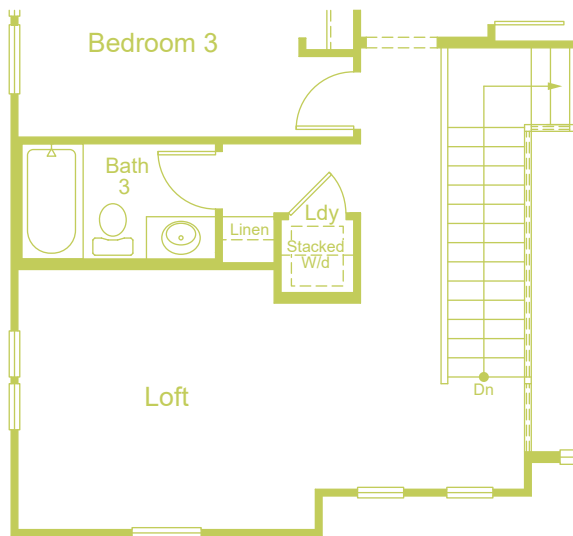
OPT. LAUNDRY 1
