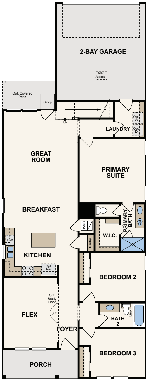
FIRST FLOOR
