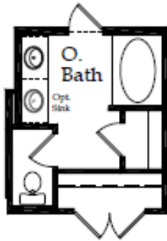
Optional Water Closet @ Owner's Bath W/ Garden Tub W/ Shower
