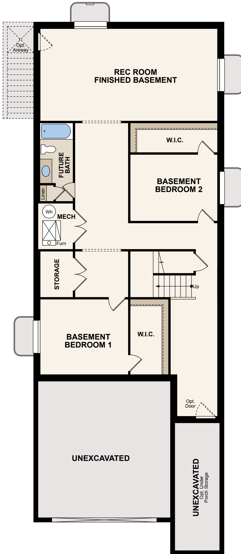
FINISHED BASEMENT
