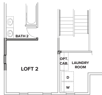
OPT. LOFT 2 AT OPT. EXPANDED GARAGE 1
