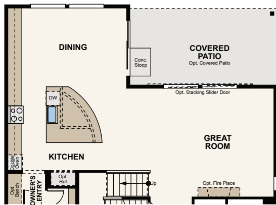
OPT. KITCHEN ISLAND & EXTENDED CABS W/ OPT. EXTENDED DINING ROOM
