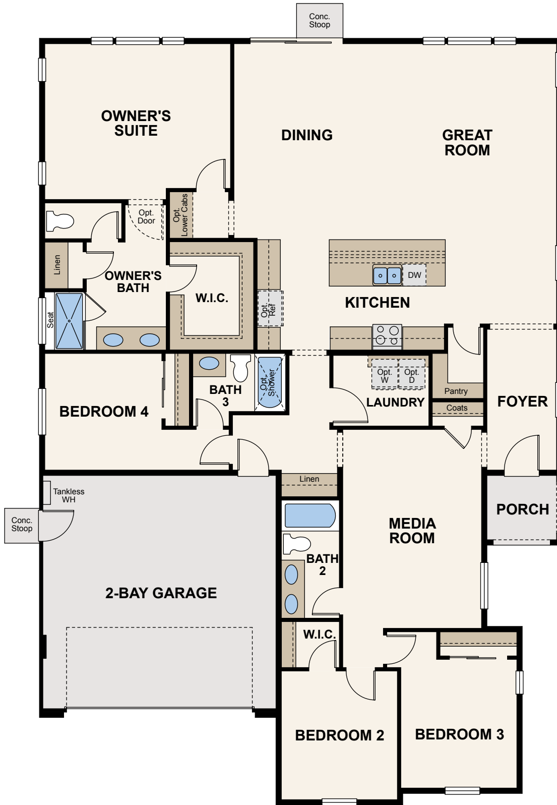
FLOOR PLAN
