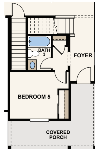
OPT. STAIRS AT BASEMENT
