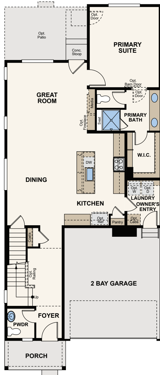
FIRST FLOOR
