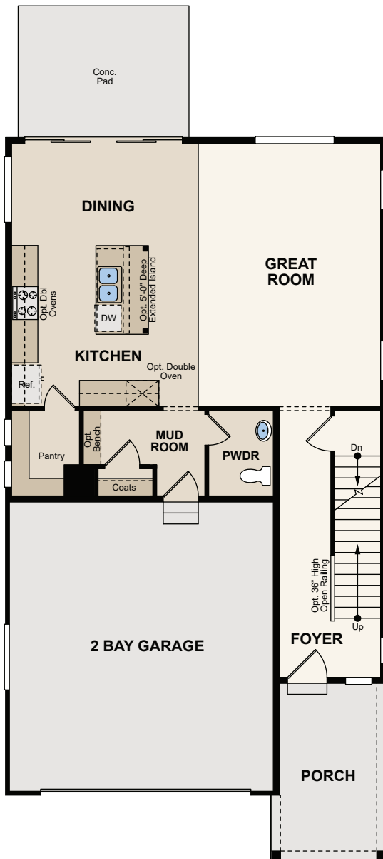
FIRST FLOOR
