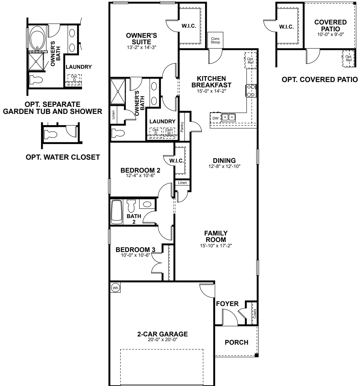
FLOOR PLAN
